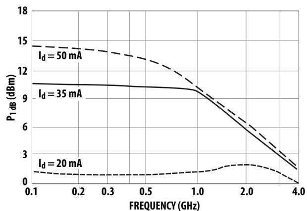
Figure 4. Output Power at 1 dB Gain Compression vs. Frequency.
